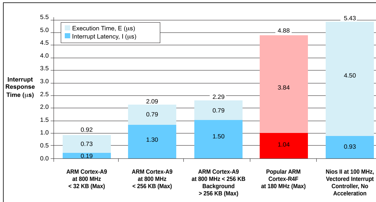
Figure 15. Interrupt Response: Nios II Solution Without Acceleration Compared to Cortex-A9 MPCore and Cortex-R4F Processors
