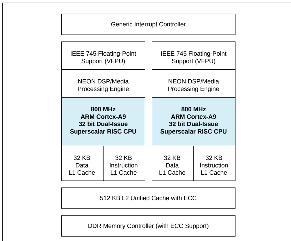
Figure 6. Dual-Core Cortex-A9 MPCore Processor on a SoC
